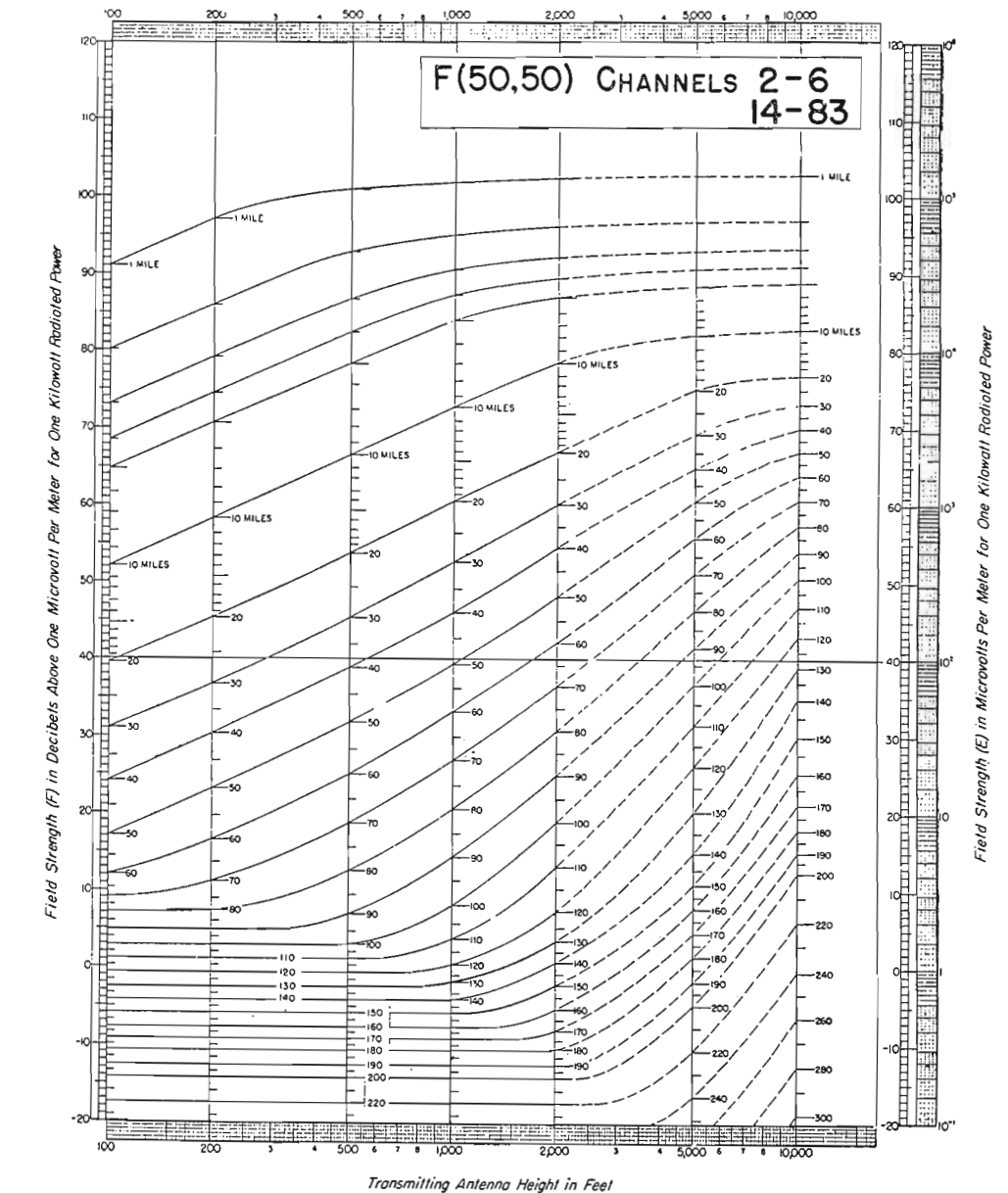
FIG. 6 (right). Reproduction of Fig. 5 of the Federal Communications Commission's "Sixth Report and Order". This is the F(50,50) Table referred to in the article. Technically, it shows the "Estimated Field Strength Exceeded at 50 Per Cent of the Potential Receiver Locations for at Least 50 Per Cent of the Time at a Receiving Antenna Height of 30 Feet". The FCC used this table in determining the "Table of Assignments" for Television Broadcasting Stations.
