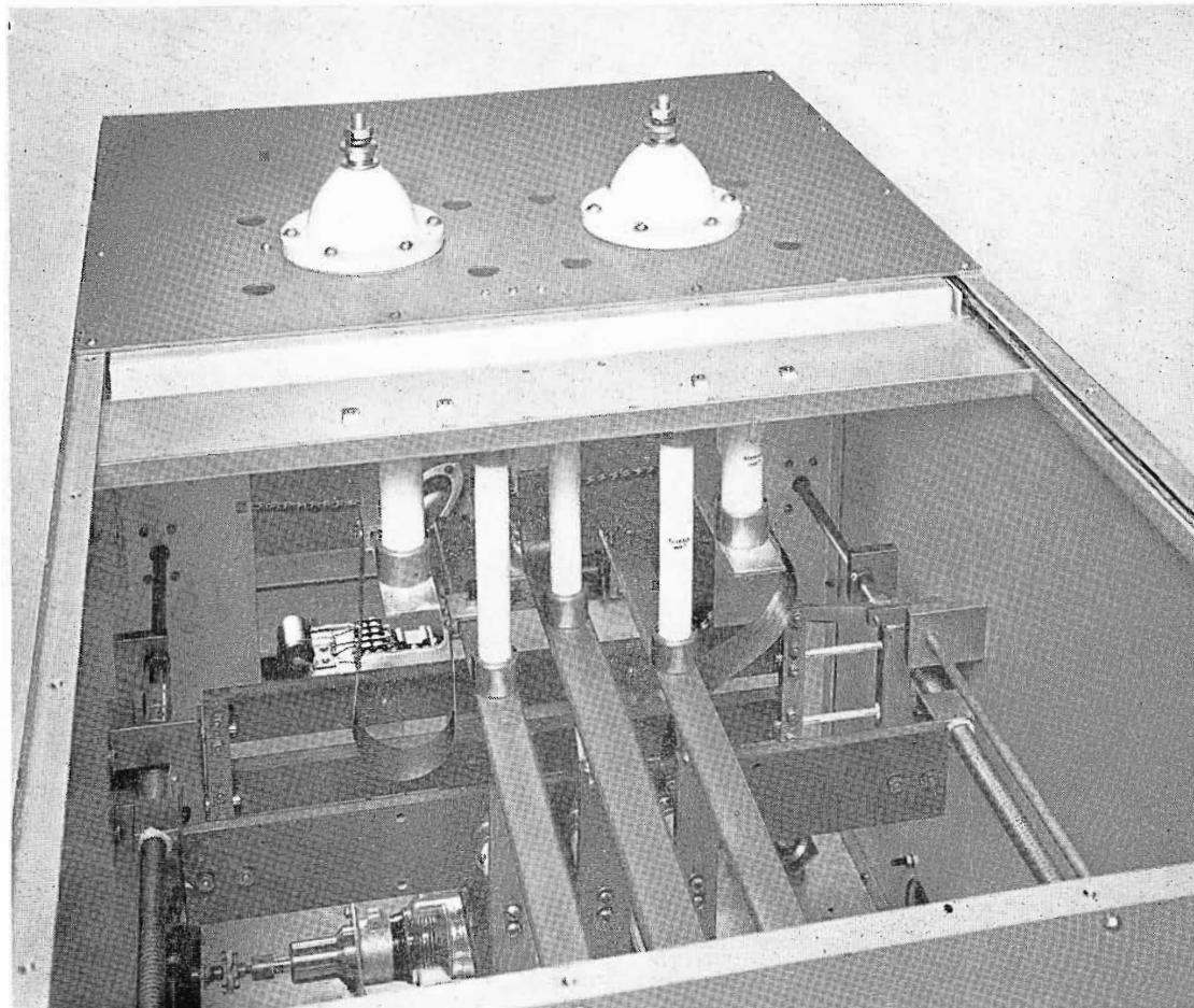
FIG. 7. Output Circuit showing inductance and tuning capacitors.
