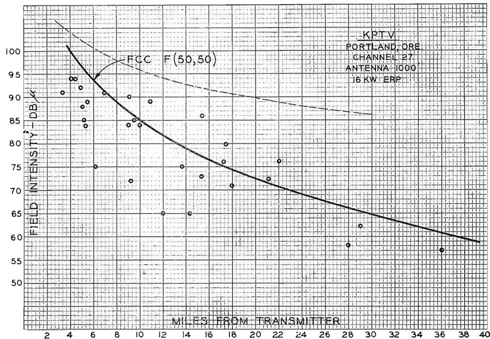
FIG. 2 (right, above). Plot of field intensities measured at KPTV, Portland, Oregon. Solid curve is from FCC's F(50,50) Table for indicated power and antenna height. Broken curve is the "free space" field strength for this power.
