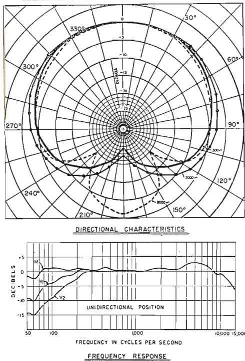
FIG. 3. RCA Type 77-D frequency response and directional pattern.
