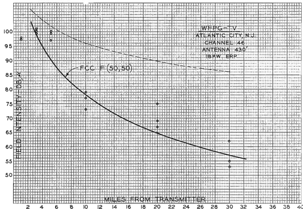
FIG. 5 (left). Plot of field intensities measured at WFG-TV, Atlantic City, New Jersey.
