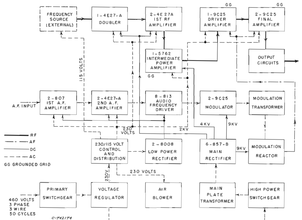
FIG. 3. Block Diagram of the BHF-50A.
