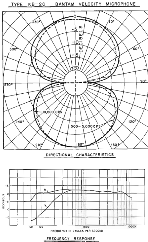
FIG. 8. KB-2C frequency response and directivity pattern.
