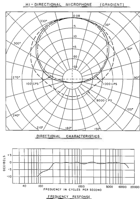
FIG. 5. Gradient microphone frequency response and directional pattern.
