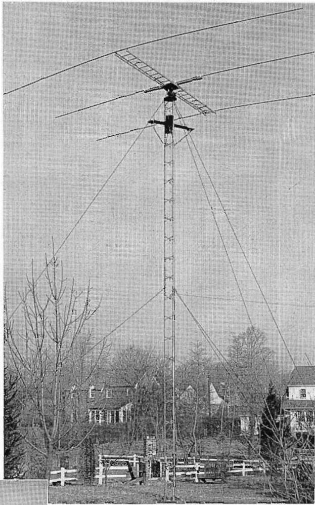
Bob's 20-meter rotary, perched on a 40-foot triangular tower, is inductively coupled to a low-impedance open-wire line.
