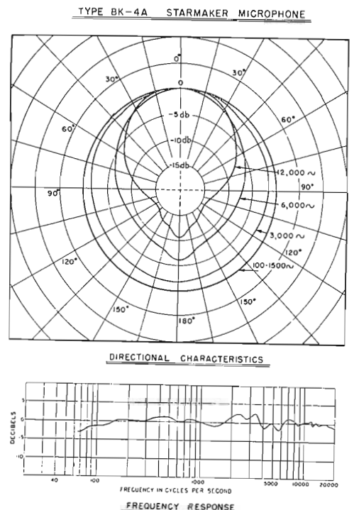
FIG. 10. BK-4A frequency response and directional pattern.
