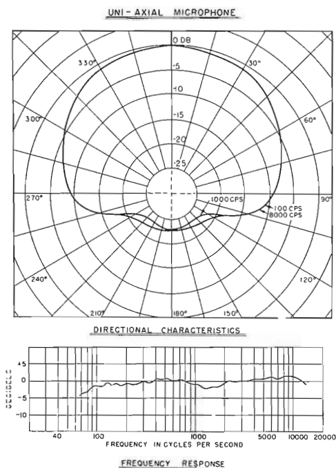
FIG. 14. Uni-axial microphone directional characteristics and frequency response.
