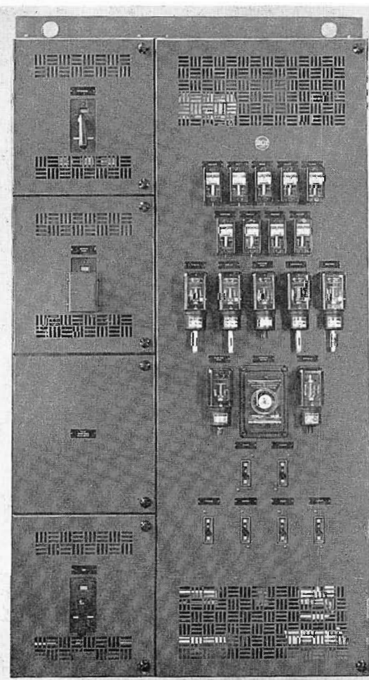
FIG. 13. Power Distribution and Control Unit showing location of overload relays.
